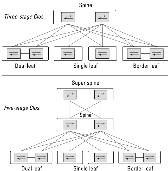
FIGURE 3-6: Three-stage and five-stage Clos designs.
