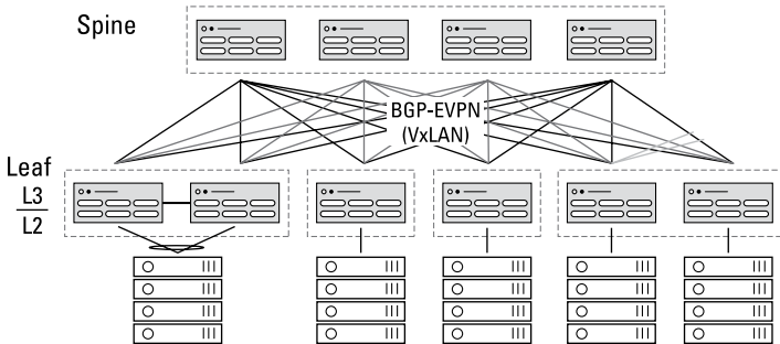
FIGURE 3-7: BGP-EVPN (VXLAN) design.
