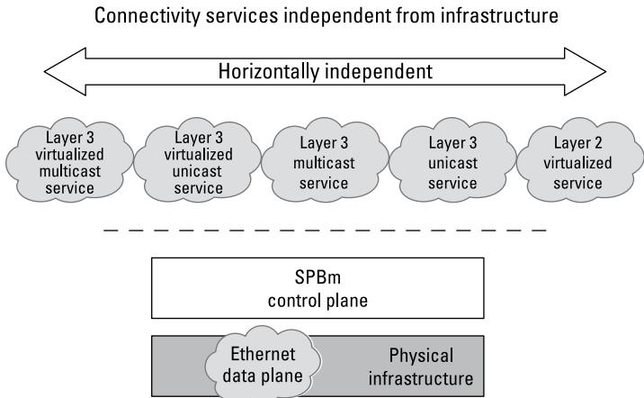
FIGURE 3-1: Shortest Path Bridging (SPB).
